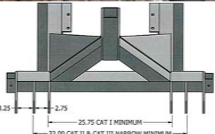
DIMENSIONS FOR HOMESTEAD 110-200
