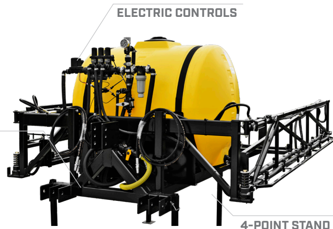
HOMESTEAD-200-EC (Boom45 w/Tip Lift)
